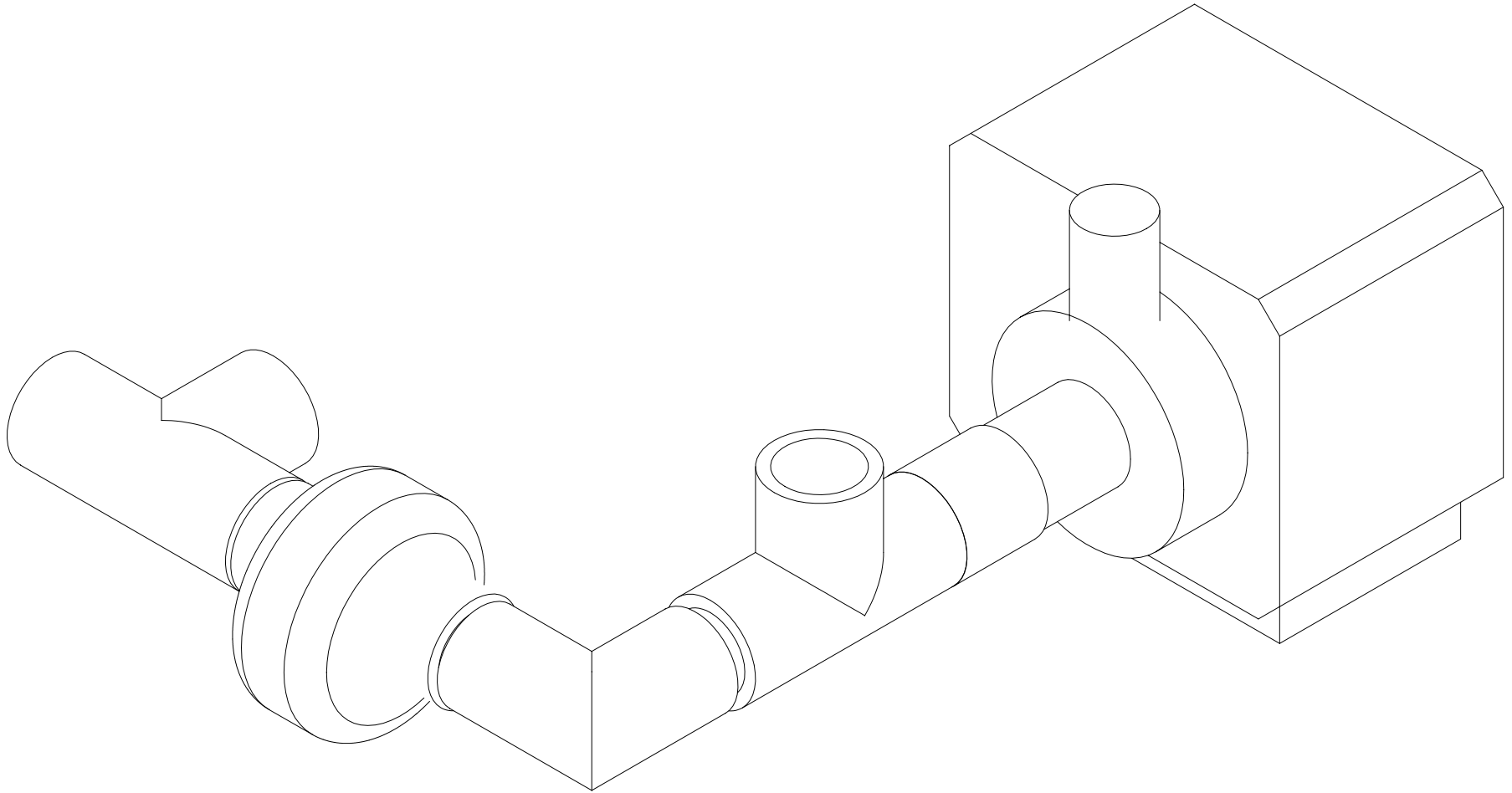
Pump Connections - Isometric View
