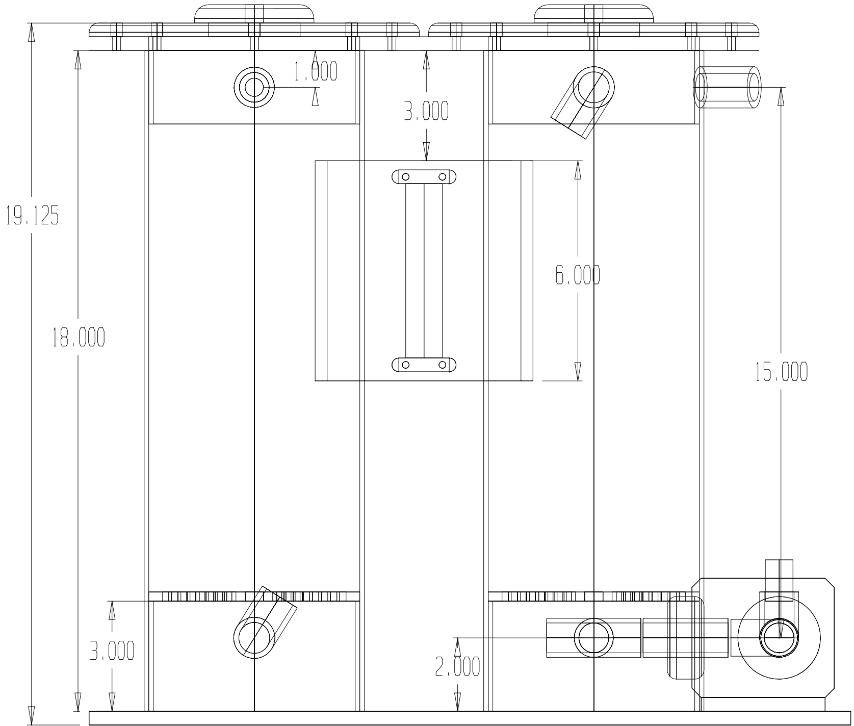
Dual Chamber Calcium Reactor - Front View
